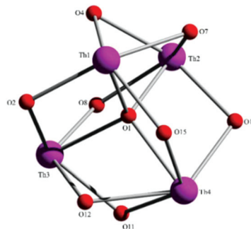
Fig. 2 The {Th 4 IV (μ 4 -O)(μ-OR) 8 } core of molecules 1 and 2. O1 is the μ 4 -O 2- group in 1, O4 and O12 are the bridging oxygen atoms of the iminiumphenolate parts of the LH - in 1 ligands, while the remaining oxygen atoms belong to the L 2- groups.
