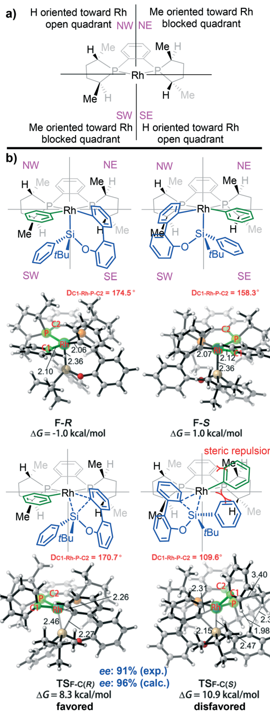
Fig. 5 (a) Quadrant analysis of the chiral environment created by the ( S,S )-Me-Duphos ligand. (b) Optimized structures of F-R , F-S , TS F-C(R) and TS F-C(S) . Distances are given in angstroms and angles in degrees.
