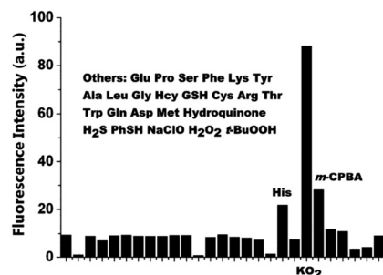
Fig. 79 Fluorescence responses of probe 53 ( 10 \mu\text{M} ) to \text{KO}_2 , \text{H}_2\text{O}_2 , \text{NaClO} , t\text{-BuOOH} , m\text{-CPBA} , hydroquinone, \text{H}_2\text{S} , \text{PhSH} , \text{GSH} , and amino acids ( 100 \mu\text{M} each) at room temperature in PBS buffer. Data were recorded at 10 min after addition of various analytes ( \lambda_{\text{ex}} = 492 \text{ nm} , \lambda_{\text{em}} = 513 \text{ nm} , slit: 2.5 \text{ nm}/2.5 \text{ nm} ). Copyright 2018 American Chemical Society.
