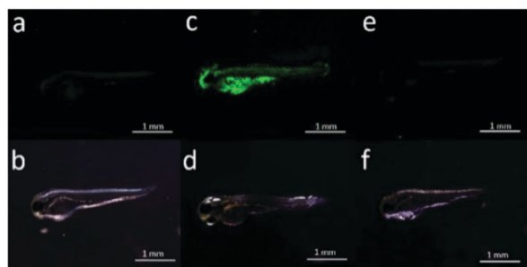
Fig. 81 Confocal imaging of endogenous \text{O}_2^{\bullet-} in 72 h post-fertilization zebrafish embryos. (a and b) Zebrafish embryos preloaded with probe 53 ( 10 \mu\text{M} ) for 20 min; (c and d) zebrafish embryos briefly challenged with PMA ( 200 \text{ ng mL}^{-1} ) for 20 min after preloaded with probe 53 ( 10 \mu\text{M} ) for 20 min; (e and f) zebrafish initially stimulated with PMA ( 100 \text{ ng mL}^{-1} ) for 20 min, treated with Tiron ( 100 \mu\text{M} ) for 20 min and loaded with probe 53 ( 10 \mu\text{M} ) for 20 min. (a, c and e): green channel, (b, d and f): bright channel. Scale bar = 1 \text{ mm} . Copyright 2018 American Chemical Society.
