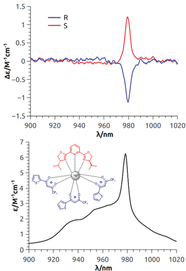
Fig. 3 Top: NIR-ECD spectra of both the enantiomers of \text{Yb}(\text{NTA})_3\text{PrPyBox} ; bottom: total NIR absorption. The spectra are measured in 7 mM \text{CH}_2\text{Cl}_2 solution (room temperature).
