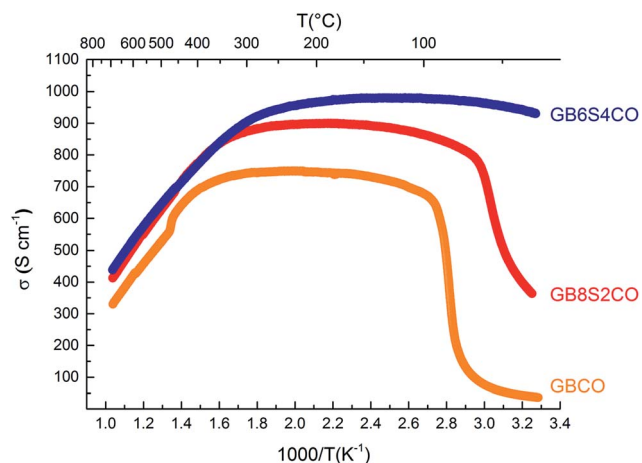
Fig. 8 Total DC electrical conductivity of GBCO (orange), GB8S2CO (red) and GB6S4CO (blue) as a function of temperature showing higher conductivity was achieved for higher Sr-doped sample.
