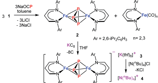
Scheme 1 Synthesis of molecular precursor 2 and its reactivity.
