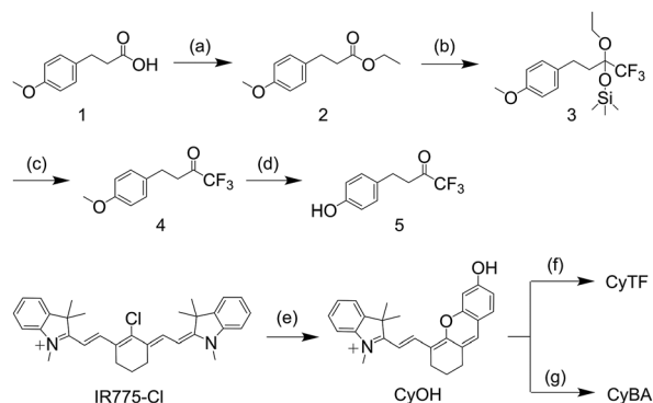
Scheme 2 Synthetic route of CyTF and CyBA . (a) \text{H}_2\text{SO}_4 (con.), reflux, 4 h, EtOH, 97%; (b) \text{TMSCF}_3 , CsF, THF, 18 h, 86%; (c) \text{TBAF} , THF, 5 h, then 4 M HCl, 3 h, 97%; (d) \text{BBr}_3 , -78^\circ\text{C} , room temperature, 12 h, \text{CH}_2\text{Cl}_2 , 74%; (e) \text{K}_2\text{CO}_3 , resorcinol, \text{CH}_3\text{CN} , 2 h; (f) 5 , \text{BTC} , \text{Et}_3\text{N} , 0^\circ\text{C} , 2 h, \text{CH}_2\text{Cl}_2 , 28%; (g) 4-methylphenylboronic acid pinacol ester, \text{K}_2\text{CO}_3 , \text{CH}_3\text{CN} , 75%.
