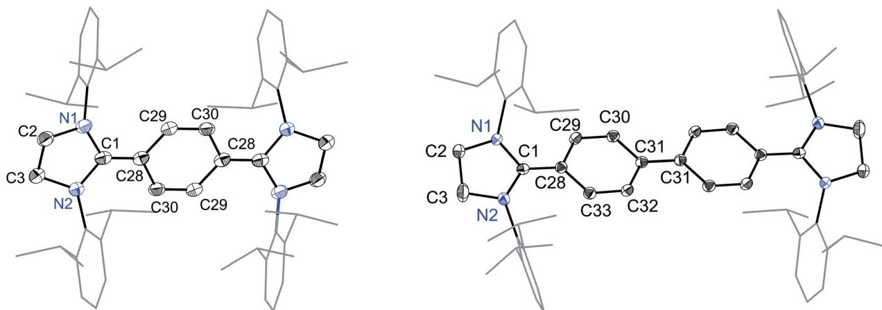
Fig. 4 Solid-state molecular structures of [(\text{SiPr})(\text{C}_6\text{H}_4)(\text{SiPr})] (4) (left) and [(\text{SiPr})(\text{C}_6\text{H}_4)_2(\text{SiPr})] (5) (right). Hydrogen atoms have been omitted for clarity. Selected bond lengths and angles for 4 and 5 are given in Table 1.
