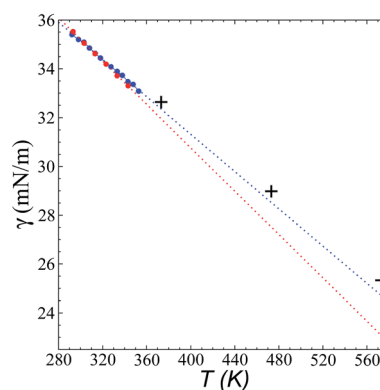
Fig. 8 Surface tension of the [bmim][triflate] system as a function of temperature. Blue and red circles represent the experimental results of Součková et al. 8 and Freire et al. 9 respectively, while the crosses represent the results of this work. Dashed lines represent linear extrapolations of the experimental data.
