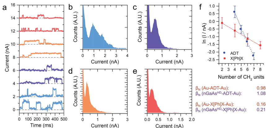
Fig. 3 (a) Example I(t) traces for nGaAs HD –X[Ph]X–Au junctions. Traces are offset on the y axis for clarity. (b) Histogram constructed from 1154 individual current jumps for nGaAs HD –1[Ph]1–Au junctions. (c) Histogram constructed from 532 individual current jumps for nGaAs HD –2[Ph]2–Au junctions. (d) Histogram constructed from 1196 individual current jumps for nGaAs HD –3[Ph]3–Au junctions. (e) Histogram constructed from 970 individual current jumps for nGaAs HD –4[Ph]4–Au junctions. (f) Plot of current jump magnitude versus number of CH 2 units plot used to determine the value of \beta_N . All data shown in this Figure is obtained in the dark.
