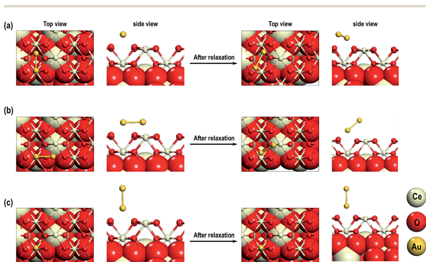
Fig. 11 \text{Au}_2 on (a) \text{M}_{\text{Au-Dim}} 1 : one of the two Au atoms on the long-bridge site and another on the 4\text{-fold}_{\text{hollow}} site, (b) \text{M}_{\text{Au-Dim}} 2 : both the Au atoms on the long-bridge site and (c) \text{M}_{\text{Au-Dim}} 3 : one of the two Au atoms is on the long-bridge site and the other above it.
