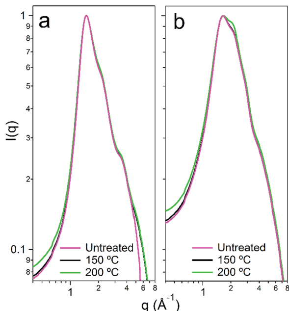
Fig. 5 WAXS data from beamline I22, Diamond Light Source, UK, showing untreated and microwave-treated samples of the pure reline-0w DES (a), and the hydrated reline-10w DES (b). Data are background-corrected and the intensity of the major correlation peak scaled to unity, to facilitate comparison and account for manufacturing variations in the X-ray capillaries used for measurement.
