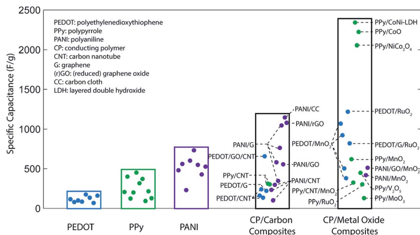
Fig. 2 Comparison of the specific capacitance of conducting polymer-based supercapacitors.
