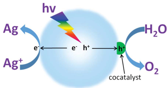
Fig. 10 Schematic illustration of photocatalytic water oxidation for \text{O}_2 evolution in the presence of an electron acceptor driven by a semi-conductor modified with \text{O}_2 evolution cocatalysts.
