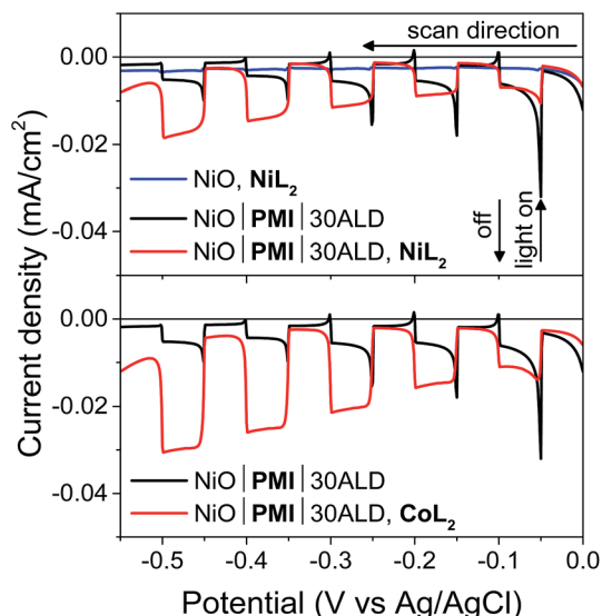
Fig. 4 Linear sweep voltammetry measurements with 10 s light on/off cycles on a NiO working electrode with 0.5 \text{ mM NiL}_2 (blue) and on a single NiO|PMI|30ALD working electrode without catalyst (black) and with 0.5 \text{ mM NiL}_2 or 0.5 \text{ mM CoL}_2 (red) (conditions: 0.1 \text{ M H}_2\text{SO}_4 and 0.1 \text{ M Na}_2\text{SO}_4 in 1 : 1 \text{H}_2\text{O} : MeCN, 5 \text{ mV s}^{-1} ).
