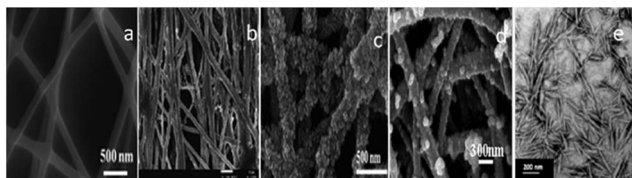
Fig. 1 SEM images of various types of CNF synthesized from cotton (a) natural electrospun CNF 56 (b) aligned CNF (scale bar 1 μm) 54 (c): CdS functionalized CNF 53 (d): CeO 2 functionalized CNF 56 (e): CNF prepared by acid hydrolysis 52 (adopted with permission).
