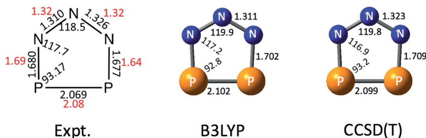
Fig. 2 Comparison of the X-ray structure of P_2N_3^- in [Na-kryptofix-221][ P_2N_3 ] salt (major component in black, minor component in red) 27 with the calculated structures at B3LYP/aug-cc-pVTZ and CCSD(T)/aug-cc-pVTZ levels of theory. Bond distances are in angstroms (Å) and bond angles are in degrees (°).
