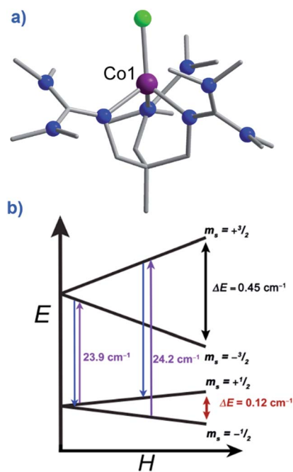
Fig. 21 (a) Molecular structure of [(3G)CoCl](CF 3 SO 3 ) ( 58 ). Colour code: purple (Co), bright green (Cl), blue (N), grey (C). Hydrogen atoms omitted for clarity. (b) Zeeman splitting diagram for 58 , where the red arrows indicated the direct relaxation process, the purple arrows correspond to the excitation energies related to the Orbach processes, and the blue arrows correspond to the relaxation via the Orbach process. All values presented were determined for S = 3/2 , g , D , and E as determined by EPR spectroscopy. Reprinted with permission from ref. 65. Copyright (2012) Royal Society of Chemistry.
