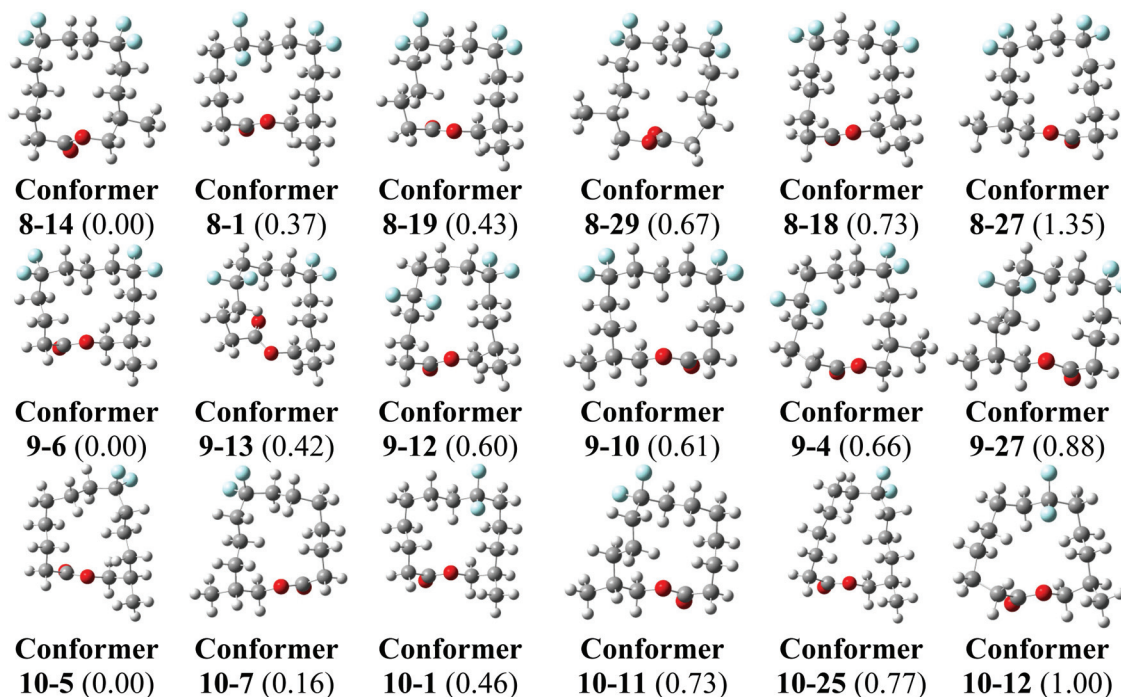
Fig. 7 The calculated lowest energy geometries for 8, 9 and 10. Relative Gibbs free energies calculated at the B3LYP-D3/6-311+G** level in kcal mol -1 are given between parenthesis. For full details see ESI.†
