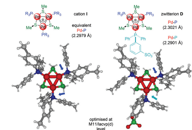
Fig. 2 Comparison of optimised structures of cation I and zwitterion D; the Pd–P distances in D at the M11/lacvp(d) level vary by +0.0041 and –0.0078 Å with the neutral and anionic phosphines respectively.
