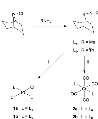
Scheme 2 Reagents: (i) [\text{PtCl}_2(\text{NC}^i\text{Bu})_2] in \text{CH}_2\text{Cl}_2 ; (ii) [\text{Cr}(\text{CO})_4(\text{nbd})] (nbd = norbornadiene) in \text{CH}_2\text{Cl}_2 .
