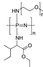
Fig. 23 Representative structure of a typical thermosensitive poly(organophosphazene). The ratio of the hydrophobic isoleucine ester versus the hydrophilic polyethylene glycol units can be used to tailor the solution properties of the polymers. Further co-substitution is used to tune the mechanical and degradation properties.
