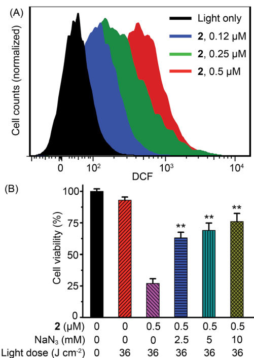
Fig. 8 (A) Analysis of ROS generation by flow cytometry during 2-mediated PDT with a ROS probe, DCF-DA. A549 cells were irradiated with a 425 nm LED light for 15 min (36 \text{J cm}^{-2} ). (B) Concentration-dependent inhibition of \text{NaN}_3 on cell death induced by 2-mediated PDT in A549 cells. Data are represented as means \pm SD of three independent experiments. ^{***}P < 0.01 , as compared with the group treated with 2 (0.5 \mu\text{M} ) in the absence of \text{NaN}_3 .
