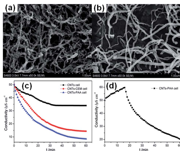
Fig. 28 SEM images of (a) CNTs and (b) CNTs-PAA composite electrodes; (c) electrodesorption process for the CNTs cell, CNTs-PAA cell and CNTs-CEM cell; (d) electrodesorption behavior for the CNTs-PAA cell under an applied voltage of -1.2 V. (Reproduced with permission from ref. 146.)
