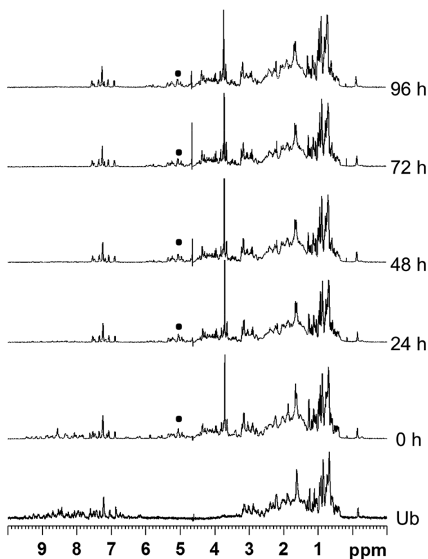
Fig. 3 ^1\text{H} NMR spectra of the mixture Ub/ [1]^{6+} (molar ratio 1:10, \text{D}_2\text{O} , 37^\circ\text{C} ) recorded between 0 h and 96 h. The ^1\text{H} NMR spectrum of free ubiquitin is shown as reference at the bottom. The p -cymene resonances of the metallaprism are labelled by (■).
