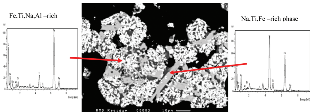
Fig. 9 The microstructure (10 \mu\text{m} ) of porous insoluble residues left after alkali roasting of bauxite and red mud at 775 ^{\circ}\text{C} in air and leaching with hot distilled water above 50 ^{\circ}\text{C} . Time of roasting – 2 hours.
