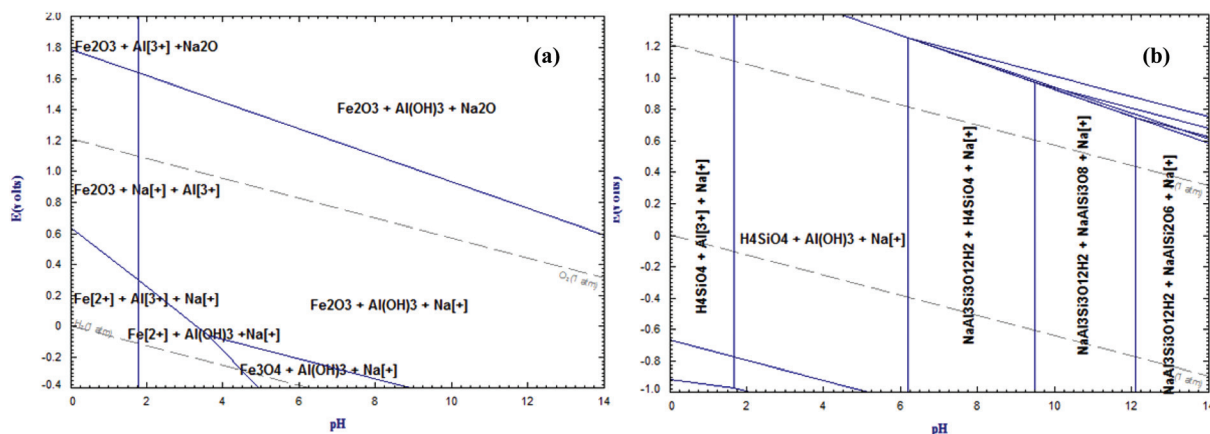
Fig. 11 (a) E_h -pH diagram of the system Na–Al–Fe– \text{H}_2\text{O} at 50 ^{\circ}\text{C} and 1 atm. (b) E_h -pH diagram of the system Na–Al–Si– \text{H}_2\text{O} at 50 ^{\circ}\text{C} and 1 atm. 66
