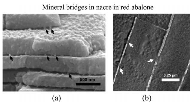
Fig. 5 TEM images of the red abalone nacre cross-section showing (a) mineral bridges between tile interfaces and (b) mineral bridges between tablets of neighboring layers shown by arrows. 79 These mineral bridges are also found in bivalves.
