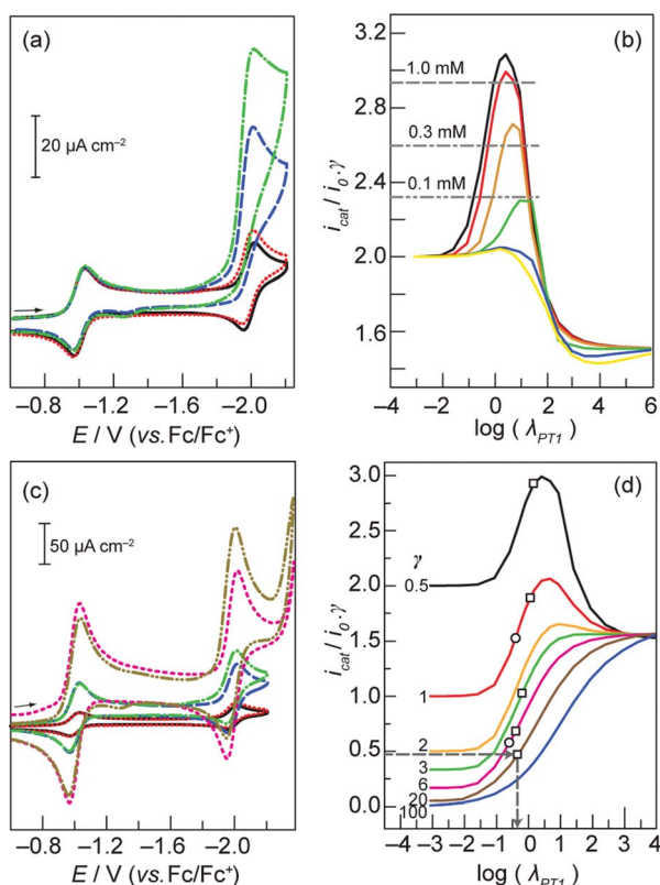
Fig. 3 (a) CVs of a 0.1 mM solution of 3 in the absence of benzoic acid (—) and in the presence of 0.05 (•••••), 0.3 (—•—), and 0.6 (—••) mM benzoic acid. Scan rate, 30 mV s -1 ; 0.2 M TBAPF 6 in acetonitrile. Glassy carbon working electrode, Ag/AgNO 3 reference electrode, and Pt wire counter electrode. (b) Working curves generated by simulating CVs with \gamma = 0.5 and \rho = 100 (—), 10 (—•—), 1 (—•—), 0.1 (—•—), 0.01 (—•—), and 0.001 (—•—). Horizontal lines indicate normalized current values ( i_{cat}/i_0\gamma ) obtained at the designated porphyrin concentrations, with half an equivalent of benzoic acid. (c) CVs of 0.1 (—), 0.3 (—•—), and 1 mM (—••) solutions of 3 in the absence of benzoic acid and in the presence of 0.05 (•••••), 0.15 (—•—), and 0.5 (—••) mM benzoic acid, respectively. Scan rate, 30 mV s -1 ; 0.2 M TBAPF 6 in acetonitrile. Glassy carbon working electrode, Ag/AgNO 3 reference electrode, and Pt wire counter electrode. (d) Working curves generated by simulating CVs with \rho = 10 . Experimental data points for 3 (□) and 2 (○) acquired at scan rates of 30 and 100 mV s -1 respectively.
