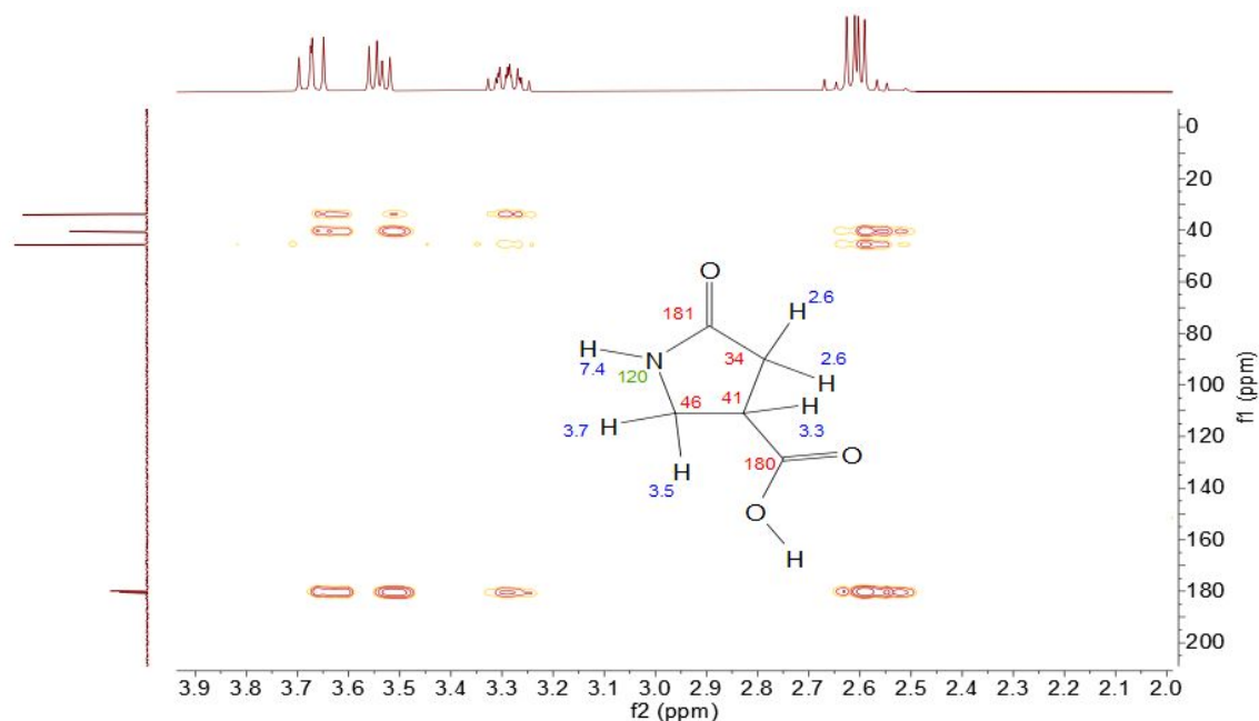
Figure 1. ^1\text{H} - ^{13}\text{C} HMBC spectra taken in \text{D}_2\text{O} and the chemical structure with NMR assignments of 1 isolated from CD dialysate. Chemical shifts of proton, carbon and nitrogen are labeled in blue, red and green, respectively.
