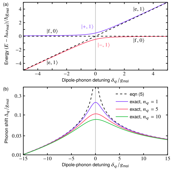
Fig. 1 DPQL with one molecule and one atom. For the eigenvectors |+, 1\rangle and |-, 1\rangle of eqn (2), the normalized eigenvalues of the energy are plotted in (a) as a function of normalized detuning \delta_q = \omega_q - \omega_{\text{mol}} . Far away from resonance, these eigenvectors asymptote to the uncoupled eigenvectors |f, 0\rangle and |e, 1\rangle . If one starts with normal mode frequency \omega_q far below \omega_{\text{mol}} in the |f, 0\rangle state and sweeps \omega_q adiabatically through resonance until it is much larger than \omega_{\text{mol}} , the population will adiabatically transfer to the |e, 1\rangle state. Energies and detunings are normalized by g_{\text{mol}} , defined as |g_q| evaluated at \omega_q = \omega_{\text{mol}} . (b) We calculate the normalized quantum AC Stark shift 21 \Delta_q of normal mode q as a function of normalized detuning from resonance for several values of n_q by numerically solving eqn (1) and compare to eqn (3). In the far-detuned limit, the shift is independent of n_q and eqn (3) is valid. The shift is asymmetric about \delta_q = 0 due to the \omega_q -dependence of g_q .
