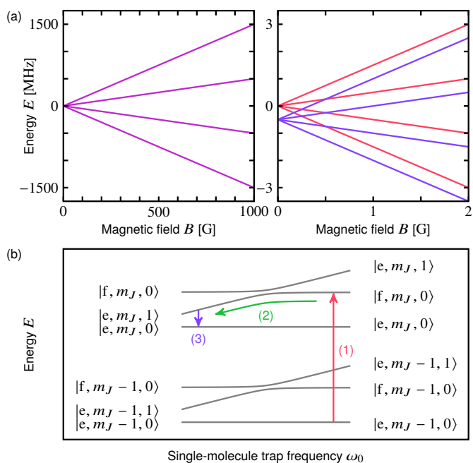
Fig. 6 Qubit state preparation. (a) Zeeman shift of \text{CaO}^+ , X^2\Pi_{3/2} , J=3/2 (left panel). The right panel shows a zoomed part of the left panel with a visible \Lambda -doublet splitting. In the right panel, f and e parities are indicated by red and blue colors, respectively. (b) The procedure of qubit state preparation. Assume the initial population is cooled to motional ground state of e parity. (1) Utilize a \sigma^+ microwave pulse to move the population from |e, m_J - 1, 0\rangle to |f, m_J, 0\rangle . In the ket, there are three notations, which correspond to parity, projection of total angular momentum, and number of phonons, respectively. (2) Adiabatically sweep the normal mode frequency across the \Lambda -doublet splitting to transfer all the \text{CaO}^+ populated in |f, m_J, 0\rangle to |e, m_J, 1\rangle . (3) Apply sideband cooling to cool \text{CaO}^+ back to motional ground state. By repeating these steps, \text{CaO}^+ can be accumulated in stretched state of e parity ( |e, m_J = 3/2, 0\rangle ). For this procedure, 800 G uniform bias magnetic field can be applied to break the degeneracy of sublevels.
