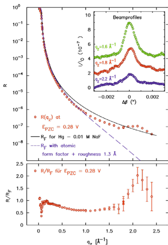
Fig. 3 (a) X-ray reflectivity of the interface between liquid Hg and 0.01 M NaF solution at a potential of 0.28 V relative to the potential of zero charge. In addition to the XRR data the Fresnel reflectivity R_F(q_z) of an ideal sharp interface and of an interface profile broadened by 1.3 \text{ \AA} roughness and the Hg atomic form factor is shown. The peak at 2.2 \text{ \AA}^{-1} indicates Hg surface layering. In the inset profiles of the reflected beam at selected q_z positions are displayed (measured at \phi = 0.05 \text{ V} ) (b) Fresnel normalized reflectivity curve of the XRR data (after Ref. 34).
