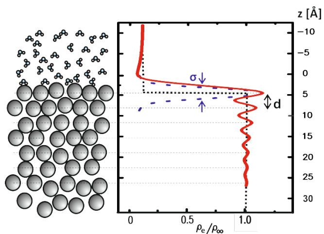
Fig. 1 Atomic-scale structure and corresponding density profile of a liquid-liquid interface.
