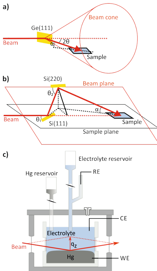
Fig. 2 Liquid interface scattering geometry with a) a single deflecting crystal and b) a double crystal Bragg deflector. c) Electrochemical cell for X-ray scattering studies of liquid metal - electrolyte interfaces. The X-ray beam enters and leaves the cell through glass windows and passes through the bulk of the electrolyte solution before and after reflection at the Hg surface. The entire cell is kept in inert gas atmosphere to keep the electrolyte clean and free of oxygen.
