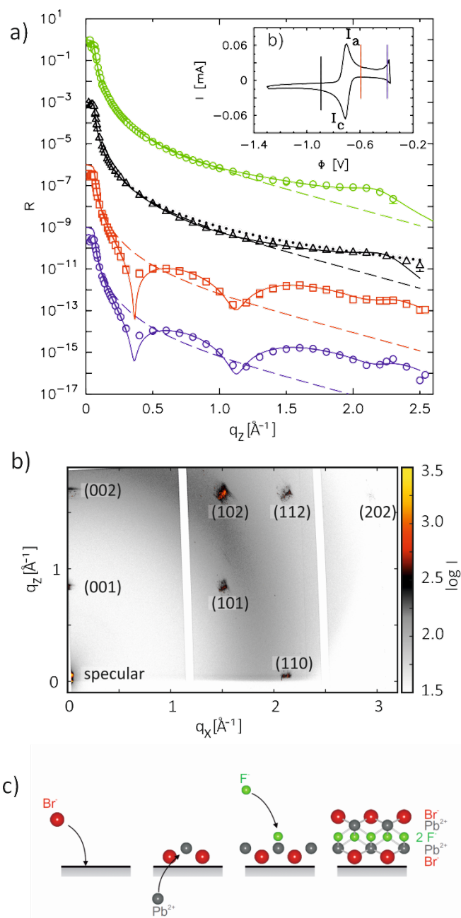
Fig. 5 In situ X-ray scattering studies of nucleation and growth on liquid Hg in 0.01 M NaF + 0.01M NaBr + 0.25 mM PbBr 2 solution. (a) Measured XRR curves at -0.90 V (black triangles), -0.60 V (red squares), and -0.40 V (blue circles) as well as an XRR curve measured at the Hg - 0.01 M NaF interface at -0.90 V (green circles). For clarity, the XRR curves are offset by a factor of 10^{-3} . Solid lines correspond to the best fits by the models described in the text, the dashed lines to the reflectivity of an interface with a Gaussian roughness of \sigma = 1.00 \text{ \AA} . (b) Corresponding cyclic voltammogram (scan rate 5 mV/s), with vertical lines marking the potentials of the XRR measurements. (c) Intensity maps in the q_y - q_z plane measured at -0.60 V \alpha = 0.135^\circ , showing Bragg reflections from a thin film of crystalline PbBrF on the Hg surface. (d) Schematic
