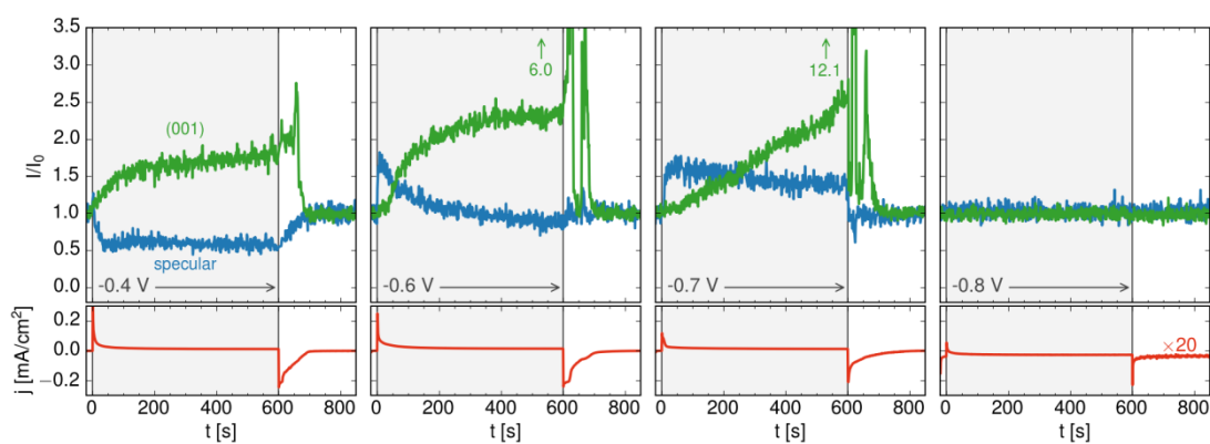
Fig 6 Kinetic studies of PbFBr growth and dissolution on Hg in 0.01 M NaF + 0.01M NaBr + 0.25 mM PbBr 2 by operando X-ray scattering. Shown is the time dependent behaviour of the specular XRR signal at q_z = 0.9 \text{ \AA}^{-1} , (blue), of the PbFBr(001) Bragg peak (green) and of the simultaneously measured electrochemical current density (red) at four different potentials (after Ref. 36).
