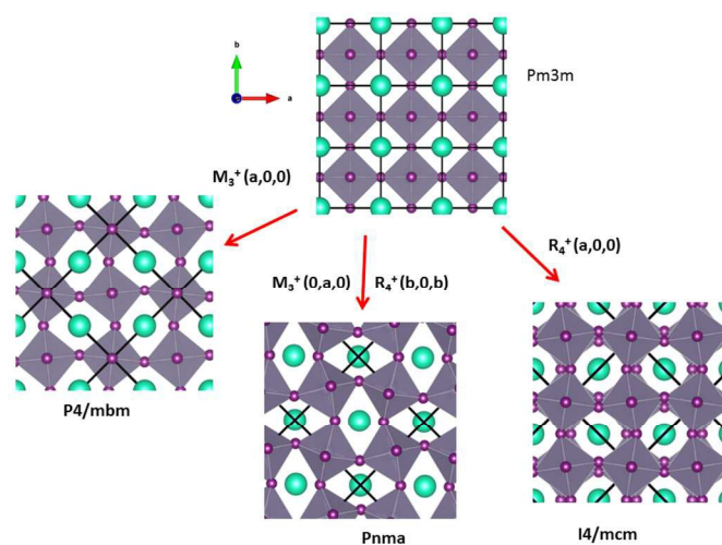
Fig. 8. Schematic representation of possible antiferro-distorsive phase transitions of AIP and HOP from the \text{Pm-3m} cubic phase. M_3^+ and R_4^+ IR define octahedra tiltings. Cations are represented by green spheres.
