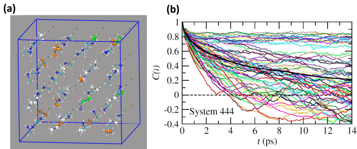
Fig. 10. (a) Atomistic representation at T=400K of the 444 supercell restricted to the CH 3 NH 3 + cations. (orange) cations having a very short relaxation time ( \tau < 1 ps), (green) cations with average relaxation time, (white) cations almost frozen on the time scale of the simulation ( \tau > 14 ps). (b) Time dependence of the autocorrelation function for all molecules within the 444 supercell extracted from MD simulation at T=400K. The average time dependence (Fig. 5 and 6) is plotted in bold dark for comparison.
