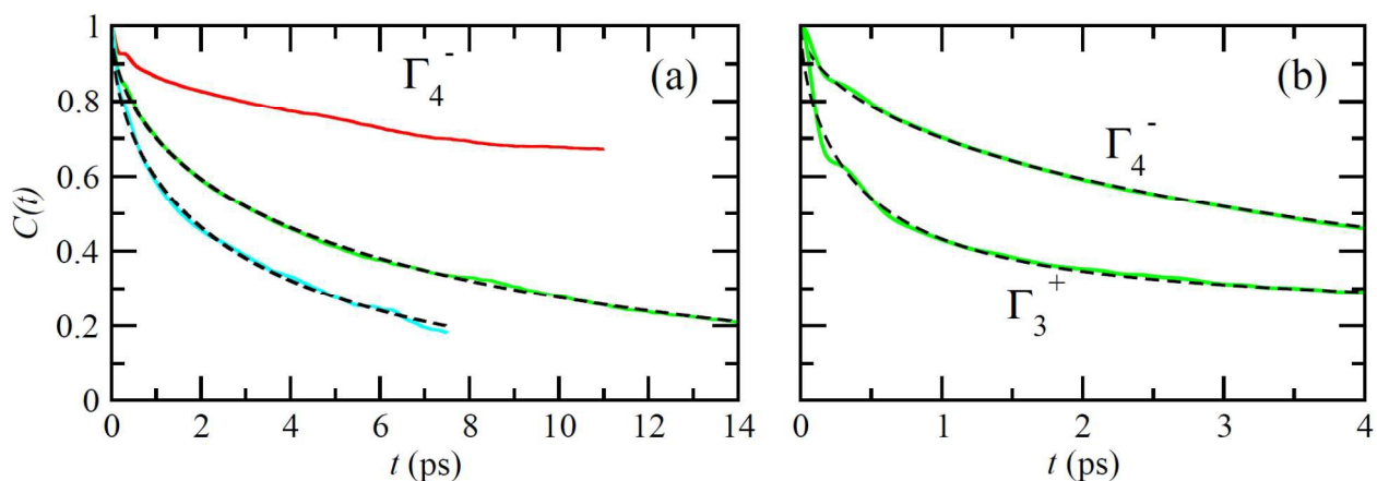
Fig. 6. (a) Temperature dependence of the average autocorrelation function of the CN axis orientation ( \Gamma_4^- ) in MAPbI 3 extracted from MD simulations for a 444 cubic supercell (solid lines): (top) 300K, (middle) 400K and (bottom) 450K. Dashed lines are fits at 400 and 450K, using stretched exponential with a stretching coefficient 0.56. (b) Detail of the initial 4 ps of the autocorrelation functions \Gamma_4^- (top) and \Gamma_3^+ (bottom) at T=400 K and corresponding fits. The relaxation times for these two curves results in a ratio \gamma_2/\gamma_1 = 1.6 .
