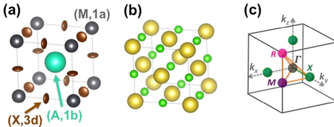
Fig. 2. (a) Simple cubic structure of \text{CH}_3\text{NH}_3\text{PbBr}_3 at high temperature. 45 The center of mass (CM) of the \text{CH}_3\text{NH}_3 (MA) cation is represented by the large green sphere, lead atoms by grey spheres. Bromide atoms exhibit anisotropically disordered motions as indicated by the brown ellipsoids. Site labels are also indicated. (b) NaCl-type structure of \text{NaCN} at high temperature. The sodium cations are represented by large yellow spheres, the CM of cyanides by small light green spheres. (c) Reciprocal space 3D view of the Brillouin Zone (BZ) with conventional labels for points of high symmetry ( \Gamma , R , M , X ).
