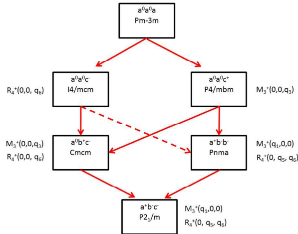
Fig. 9. Schematic diagram indicating the group-subgroup relationship between some of the space groups observed in HOP and AIP (solid red lines). The tilt systems are given using Glazer's notation, as well as the Pm-3m IR related to the lattice instabilities. The dashed red line indicates that a transition from I4/mcm to Pnma space groups must be a 1 st order phase transition.
