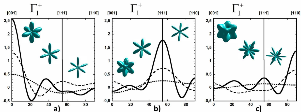
Fig. 3. Angular dependence of the probability distribution functions for molecular orientation in a local crystalline site with cubic Oh symmetry relevant for \Gamma_1^+ . \varphi=45^\circ and the \theta angle varies between 0^\circ/[001] and 90^\circ/[110] . The [111] direction is reached for \theta=54.7^\circ . The curves are given for (a) pure [001], (b) pure [111] and (c) pure [110] orderings, when the cubic harmonics expansions are considered up to K_4 (dotted lines), K_8 (dashed lines) and K_{12} (solid lines). In each panel, 3D representations of the same rotator functions are inserted considering, from left to right, expansions up to K_4 , K_8 , K_{12} , respectively.
