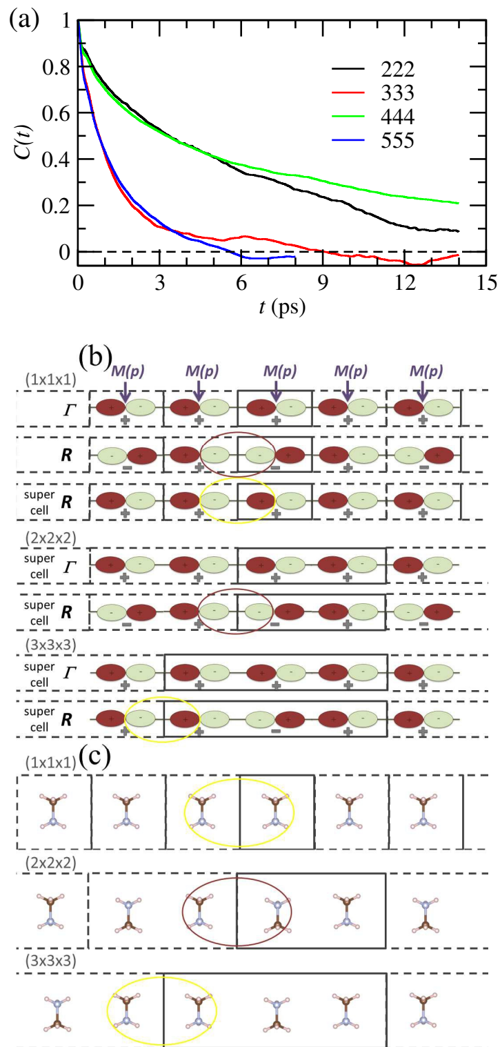
Fig. 5. (a) Time dependence of the average autocorrelation function of the CN axis orientation in \text{MAPbI}_3 extracted from MD simulation at 400K for various supercell sizes having an odd or an
