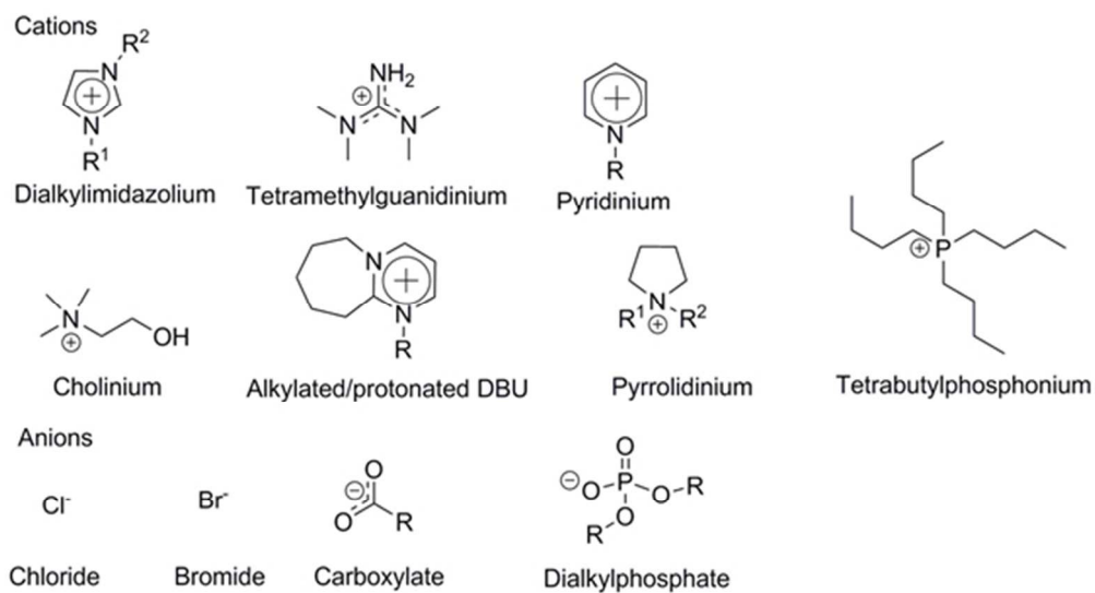
Fig. 4 Typical ion constituents of cellulose-dissolving ILs. 170x92mm (96 x 96 DPI)
