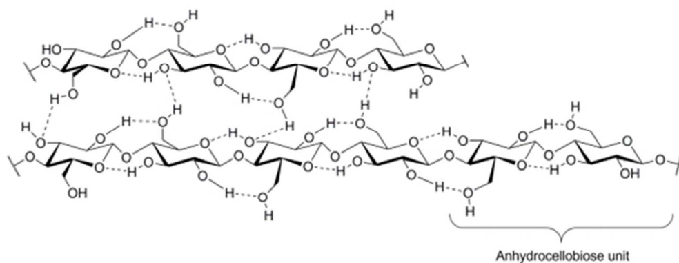
Fig. 1 Structure of cellulose and its intra- and interchain hydrogen binding. The anhydrocellobiose unit is the basic structural element of cellulose. Reproduced with permission from ref 162. 170x66mm (96 x 96 DPI)
