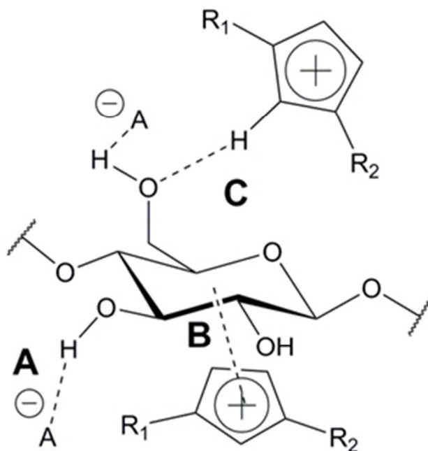
Fig. 5 Proposed dissolution mechanisms for cellulose in imidazolium-based ionic liquids: A) Interactions between the basic anion (A) and the cellulose hydroxyl groups break up the hydrogen bond network between the cellulose chains. B) Hydrophobic interactions take place between the hydrophobic face of cellulose and the imidazolium ring. C) The acidic proton at the C-2 position on the imidazolium ring interacts with the cellulose hydroxyl groups. 83x86mm (96 x 96 DPI)
