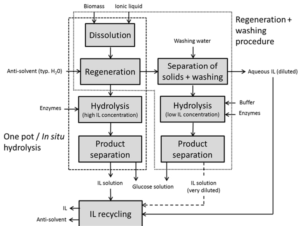
Fig 2. Processing schemes for IL pretreatment with subsequent enzymatic hydrolysis of plant cell wall polysaccharides through the one-pot and the regeneration with washing procedure. 210x157mm (96 x 96 DPI)
