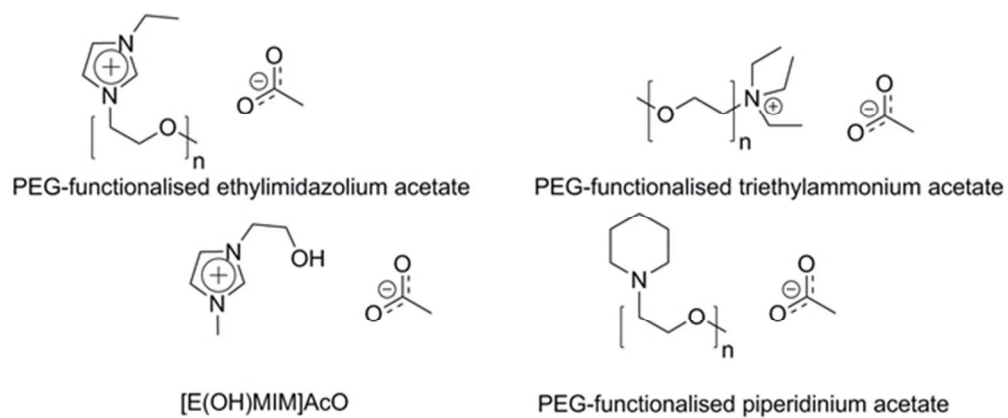
Fig. 6 Cellulose-dissolving ionic liquids designed for increased enzyme-compatibility. 170x70mm (96 x 96 DPI)
