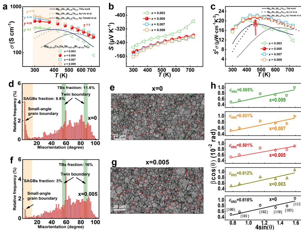
Fig. 2 The temperature-dependent electrical transport properties and microstructural evolution. The temperature-dependent electrical transport properties of Mg 3.2(1-x) Cu x Ga x Sb 1.5(1-x) Bi 0.5(1-x) Te 2x samples: (a) electrical conductivity, (b) Seebeck coefficient, and (c) power factor. The grain misorientation distributions and corresponding morphology maps for (d and e) x = 0 and (f and g) x = 0.005 samples. TBs are marked in red and SAGBs are shown in green. (h) The internal strain analysis of samples.
