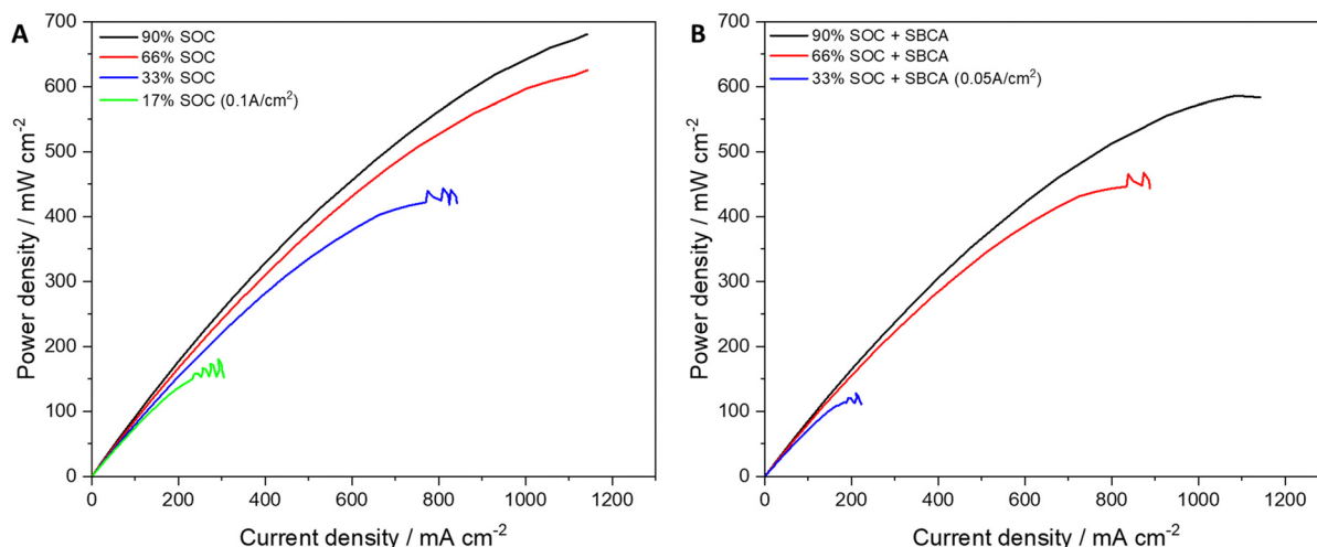
Fig. 3 RFB polarization curves at different SoC (A) before and (B) after SBCA addition.
