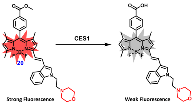
Fig. 24 Detection mechanism of probe 20 to CES1. (Redrawn the Chem-Draw structures from ref. 98).
