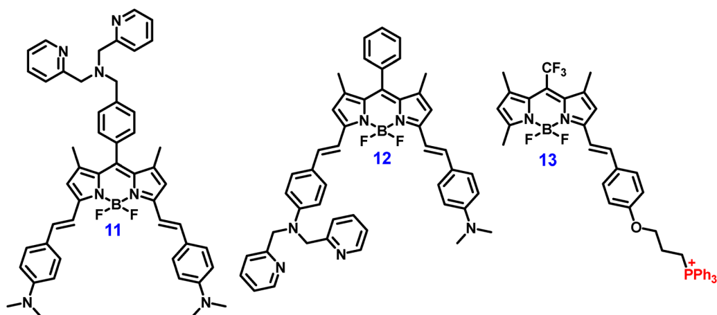
Fig. 13 Chemical structures of probes 11–13. (Redrawn the ChemDraw structures from ref. 81–83).
