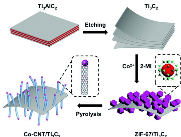
Fig. 17 Schematic illustration of the formation process for Co-CNT/ \text{Ti}_3\text{C}_2 composites. Reproduced from ref. 91 with permission from Royal Society of Chemistry, copyright © 2024.
