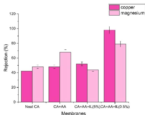
(c) Rejection performance of the membranes at a pressure of 4 bar at pH 4
