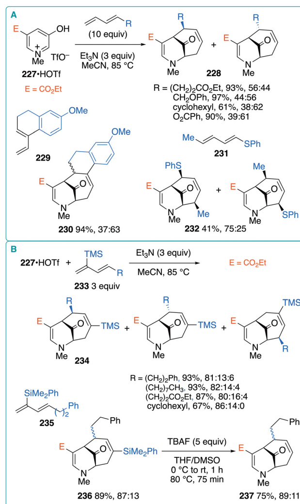
Fig. 33 (A) (5 + 4) cycloaddition of ester-substituted oxidopyridinium with unsymmetrical 1,3-dienes. (B) (5 + 4) cycloaddition of ester-substituted oxidopyridinium with dienylsilanes.
