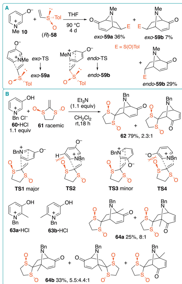
Fig. 8 (A) (5 + 2) Cycloaddition of 1-methyl-3-oxopyridinium with optically active vinyl sulfone. (B) (5 + 2) cycloaddition of 1-benzyl-3-oxopyridiniums with racemic 2-methylene-1,3-dithiolane 1,3-dioxide.
