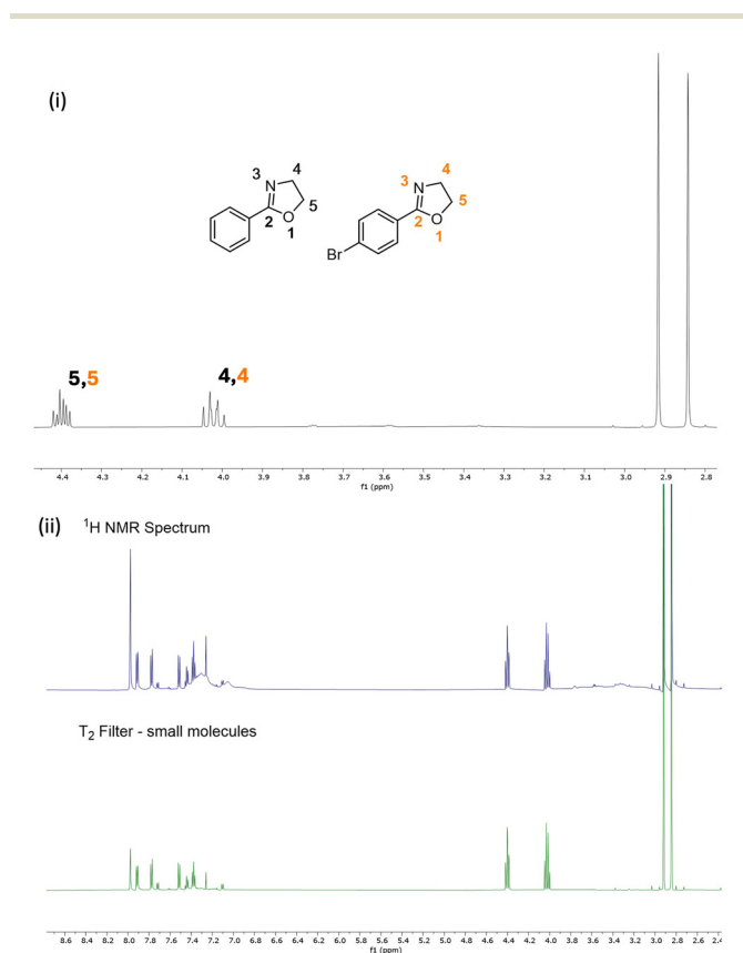
Fig. 4 (i) Partial ^1\text{H} NMR spectrum (400 MHz, \text{CDCl}_3 ) of copolymerisation of 1 and 2 , showing overlap of the signals corresponding to monomers. (ii) ^1\text{H} NMR spectrum (400 MHz, \text{CDCl}_3 ) of the same reaction mixture with T_2 filter applied.
