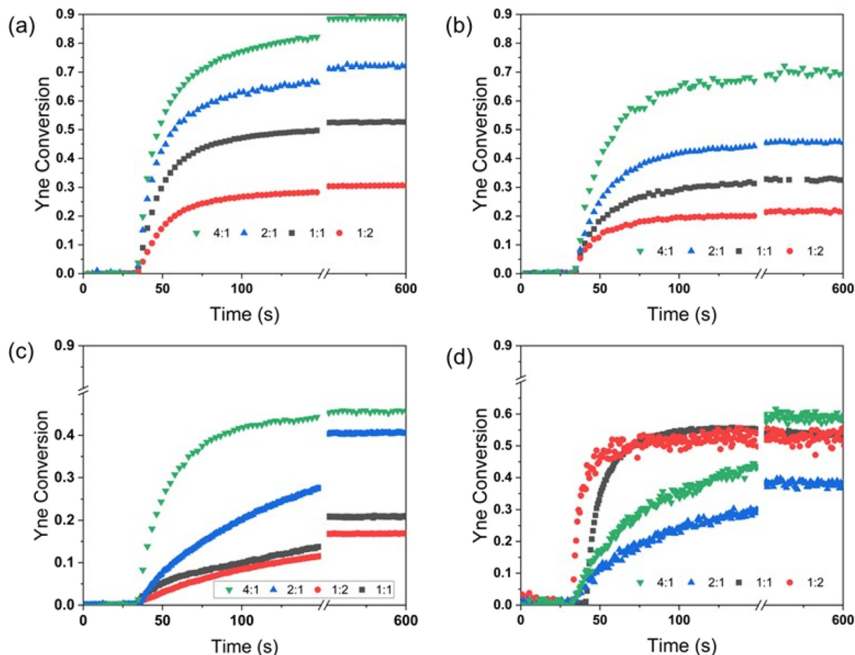
Fig. 4 FTIR conversion versus time plots for alkyne reactive groups ( \lambda = 405 nm, I = 40 mW cm ^{-2} , t = 600 s). (a) LipOMe : phenylacetylene, (b) LipOMe : 1-octyne, (c) LipOMe : propargyl acetate, and (d) LipOMe : diphenylacetylene. Black squares (dithiolane : yne = 1 : 1), red circles (dithiolane : yne = 1 : 2), blue triangles (dithiolane : yne = 2 : 1), green triangles (dithiolane : yne = 4 : 1).
