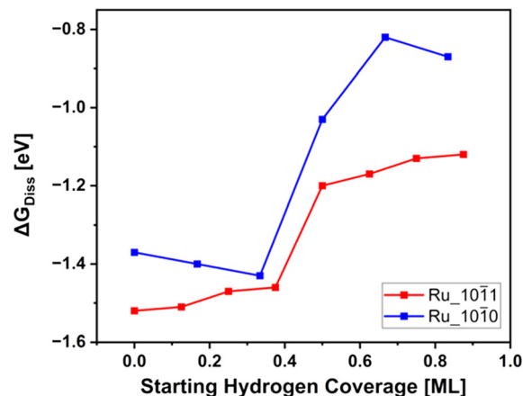
Fig. 1 \text{H}_2 direct dissociation energy ( \Delta G_{\text{Diss}} ) in eV as a function of the starting atomic hydrogen coverage ( i.e. , the coverage before the dissociation reaction) reported in monolayers (MLs) for the Ru (10 \bar{1} 1) and (10 \bar{1} 0) surfaces. Energies are reported at 0 K with ZPE corrections.
