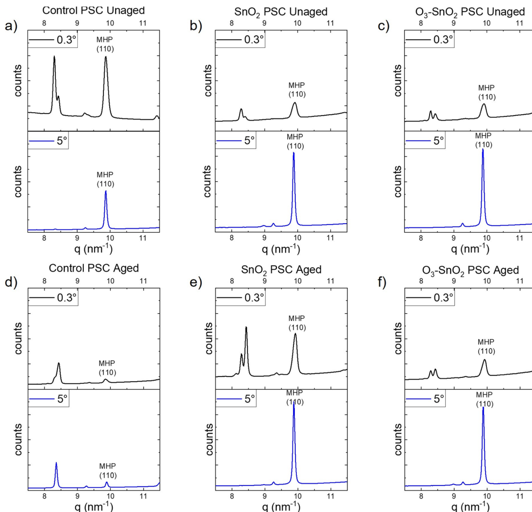
Fig. 4 Improved bulk MHP stability of PSCs with barrier layer X-ray diffraction plots in q -space at incidence angles 0.3° (representing the top surface) and 5° (representing the bulk) (a–c) unaged PSCs, and (d–f) PSCs subjected to 50 °C for 120 h. (a and d) Control PSC, (b and e) SnO 2 PSC, and (c and f) O 3 -SnO 2 PSC.
