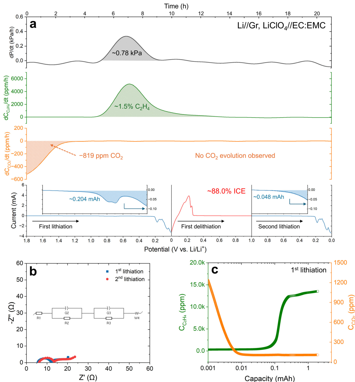
Fig. 6 Operando monitoring of gas evolution in the Li-graphite half-cell that undergoes cyclic voltammetry at a scan rate of 0.05\text{ mV s}^{-1} with 1 M LiClO_4 in EC : EMC 3 : 7 vol% as the electrolyte. (a) The obtained CV curves are plotted in conjunction with the change in concentrations of C_2H_4 , CO_2 , and in overall gas pressure. The detailed current variation from 1.8 V to 0.3 V vs. Li/Li^+ of the first lithiation and from 1 V to 0.3 V vs. Li/Li^+ of the second lithiation is provided in the insets by zooming in the y-axis. The blue shading of the first lithiation represents the electric charge consumed for the SEI formation and associated gas evolution. (b) The EIS spectra obtained after the initial and the second cathodic scan. (c) Evolution of C_2H_4 and CO_2 concentrations during the initial lithiation of graphite.
