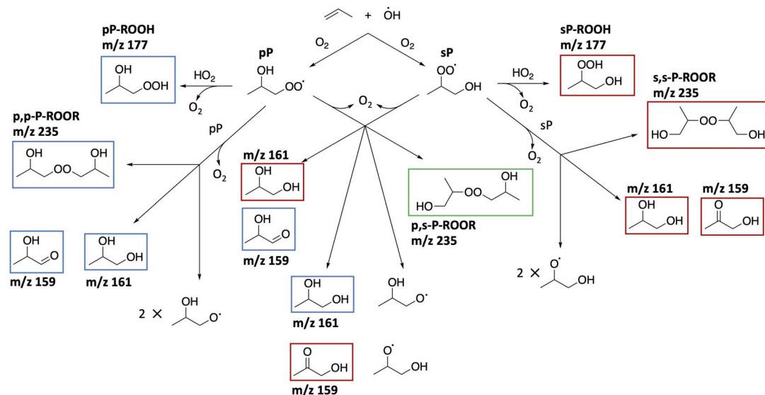
Scheme 3 Reaction scheme for the oxidation of propene by OH in the presence of O_2 . Stable products that can be observed with the CF_3O^- GC-CIMS are boxed and color-coded such that products that are derived from the primary peroxy radical are in blue, those derived from the secondary peroxy radicals are in red, and products formed from the cross-reactions of the primary and secondary peroxy radicals are in green. Each product is labelled with the m/z of that product in our CIMS, which is equal to the molecular weight + 85. In the presence of O_2 , the alkoxy radicals will form formaldehyde, acetaldehyde, and HO_2 .
