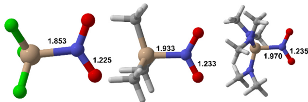
Fig. 1 Predicted geometries of selected hypothetical nitrosilanes (B3LYP/6-311+g(d,p))-SMD(acetonitrile). Left: \text{F}_3\text{SiNO}_2 ; center: \text{Me}_3\text{SiNO}_2 ; right: (\text{NMe}_2)_3\text{SiNO}_2 . Bond distances in Å. Beige = silicon, blue = nitrogen, red = oxygen, white = hydrogen, light gray = carbon, green = fluorine.
