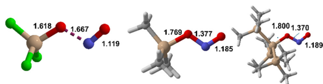
Fig. 2 Predicted geometries of selected hypothetical nitritosilanes (B3LYP/6-311+g(d,p))-SMD(acetonitrile). Left: \text{F}_3\text{SiONO} (not a stable minimum); center: \text{Me}_3\text{SiONO} ; right: (\text{Me}_3\text{Si})_3\text{SiONO} . Bond distances in Å. Beige = silicon, blue = nitrogen, red = oxygen, white = hydrogen, light gray = carbon, green = fluorine.
