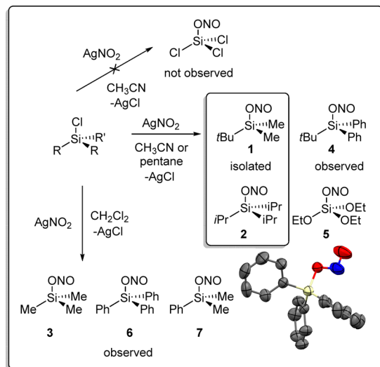
Fig. 3 Synthesis and attempted synthesis of various nitritosilanes. Bottom right: solid-state structure of 6 obtained from X-ray diffraction analysis. As expected from its slow formation in DCM, the compound co-crystallized with a small amount of the chloride starting material, which was modeled as a substitutional disorder (refined ratio ONO : Cl 0.85 : 0.15, not shown, see SI). Hydrogen atoms were omitted for clarity. Beige: silicon; dark grey: carbon; blue: nitrogen; red: oxygen.
