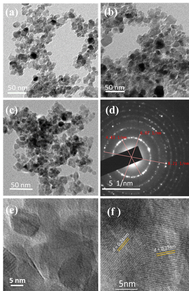
Fig. 2 TEM images of (a) TiO 2 , (b) TiCu-1, and (c) TiAg-1; (d) SAED pattern of TiAgCu-1, and HRTEM images of (e) TiAgCu-1 and (f) the lattice fringe spacing in TiAgCu-1. Ag and Cu integration on TiO 2 and the formation of a metal–semiconductor Schottky junction between Ag/Cu and TiO 2 is evident from the d -values (0.24 nm for Ag/Cu alloy formation and 0.37 nm for TiO 2 ) observed in the HRTEM image in (f).
