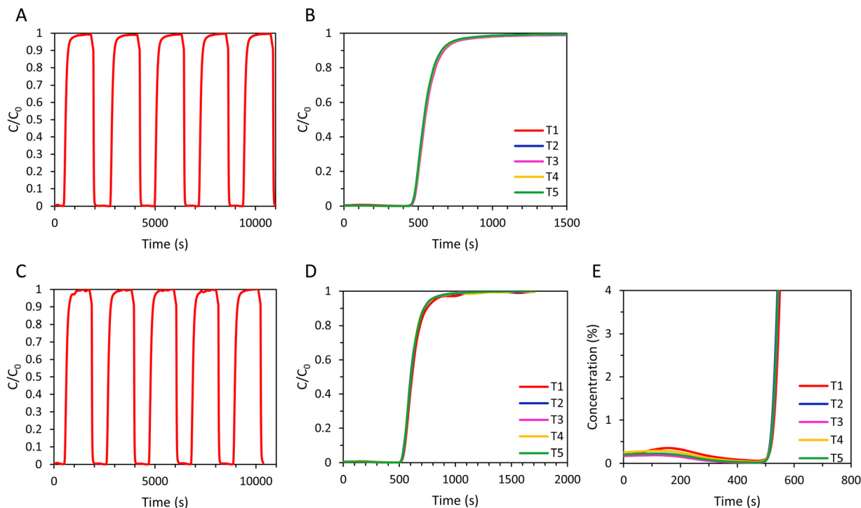
Fig. 9 (A) 5 consecutive adsorption–desorption cycles for the SAPO-34 beads in a VPSA setup, with a long desorption step; a (B) cyclic breakthrough curves of SAPO-34 beads (5 cycles), with a long desorption step; a (C) 5 consecutive adsorption–desorption cycles for the SAPO-34 beads in a VPSA setup, with a short desorption step; b (D) cyclic breakthrough curves of the SAPO-34 beads (5 cycles), with a short desorption step; b (E) cyclic breakthrough curves of SAPO-34 beads up to CO 2 concentration of 4% (5 cycles), with a short desorption step. b a Long desorption step (A) and (B): the adsorbent bed was regenerated in between cycles by evacuation at 20 mbar for 2 min, followed by flushing with N 2 until the CO 2 concentration was ≤ 0.15%. b Short desorption step (C)–(E): the adsorbent bed was regenerated in between cycles by evacuation at 20 mbar for 2 min, followed by flushing with N 2 for 139 s.
