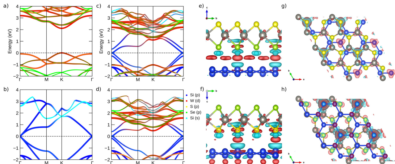
Fig. 2 The band structure projections (using HSE06) considering only orbitals that had a contribution greater than 3% of the maximum total density of states for (a) the WSe 2 Janus geometry, 58 (b) 30 degree rotated silicene, 12 (c) WSe 2 /Si and (d) WSeS/Si; (e)–(g) and (f)–(h) the side and top views of the charge density redistribution for WSe 2 /Si (WSeS/Si); \Delta\rho(\vec{r}) > 0 and \Delta\rho(\vec{r}) < 0 are represented by light red and cyan colors, respectively. Isosurface 0.0006 e Å -3 .
