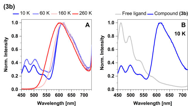
Fig. 14 (A) Steady-state luminescence spectra of 3b in cyclohexane suspension at selected temperatures of 10 K, 60 K, 160 K, and 260 K. (B) Comparison of the steady-state spectrum of 3b with the spectrum of the free ligand (4-formyl pyridine) obtained in cyclohexane solution at 10 K. The excitation wavelength was 375 nm.
